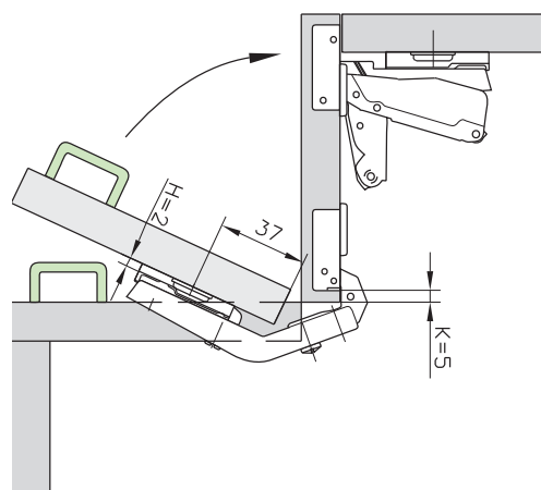
Klap šarka ugaona / ugao / FGV
