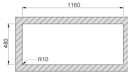
Inset Installation
